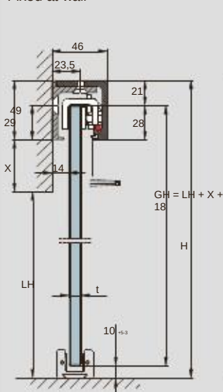
Montage mural Fixed at wall
