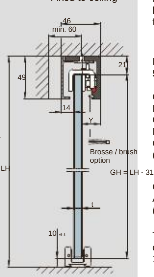
Montage plafond Fixed to ceiling
