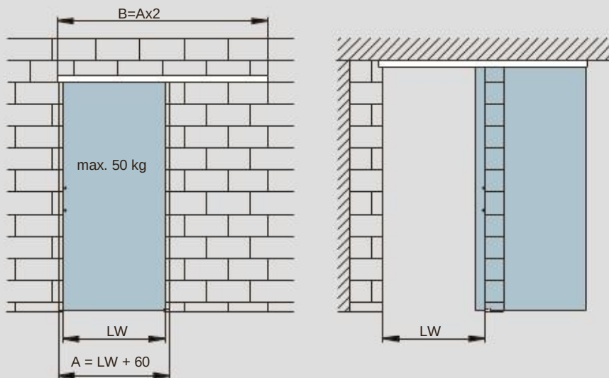
Montage mural Fixed at wall
